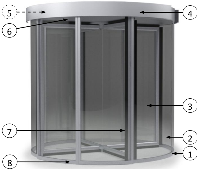
RevLock 611 + optional sliding door, non-secured area side
