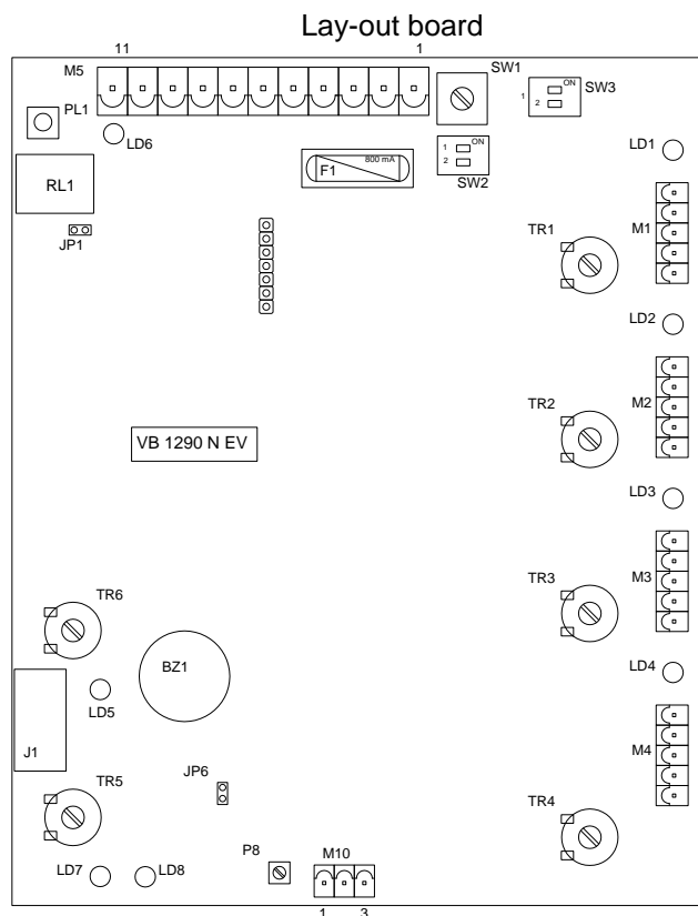
Figure 2-21 VB 1290/4 EVAM single presence board
