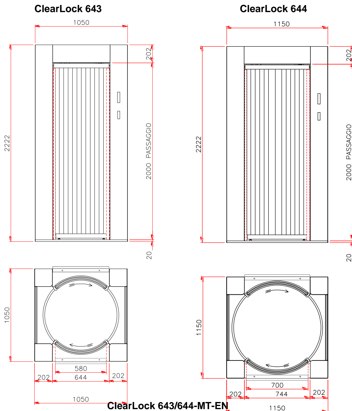
Figure 1-1 ClearLock 643 and ClearLock 644 (main dimensions)
