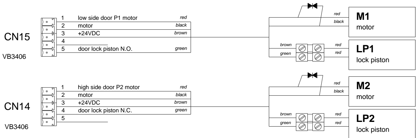
Figure 2-14 High side and low side motor and lock piston wiring
