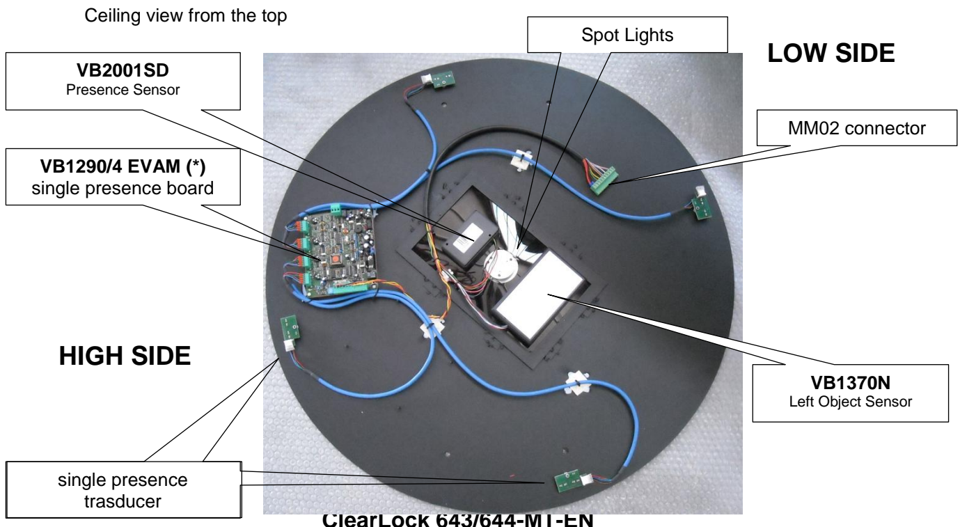
Figure 2-3 General components LAY OUT
