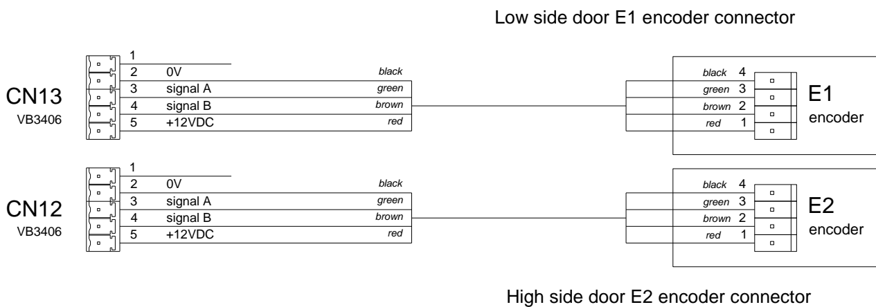
Figure 2-13 High side and low side motor encoder wiring
