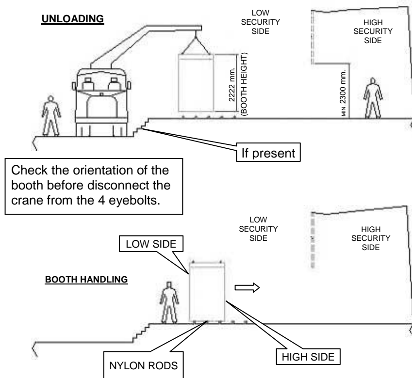
Figure 2-1 How to position the booth on the floor in order to move it
