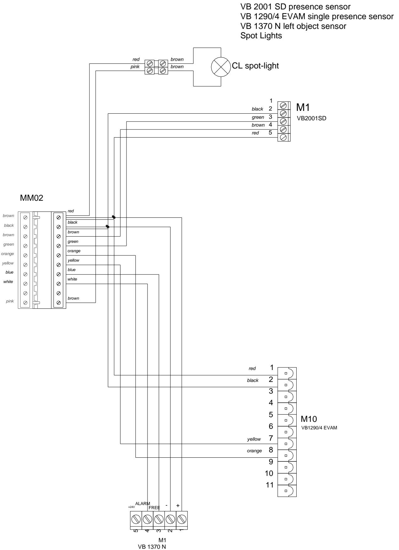
Figure 2-17 Connector MM02 wiring (part 2)
