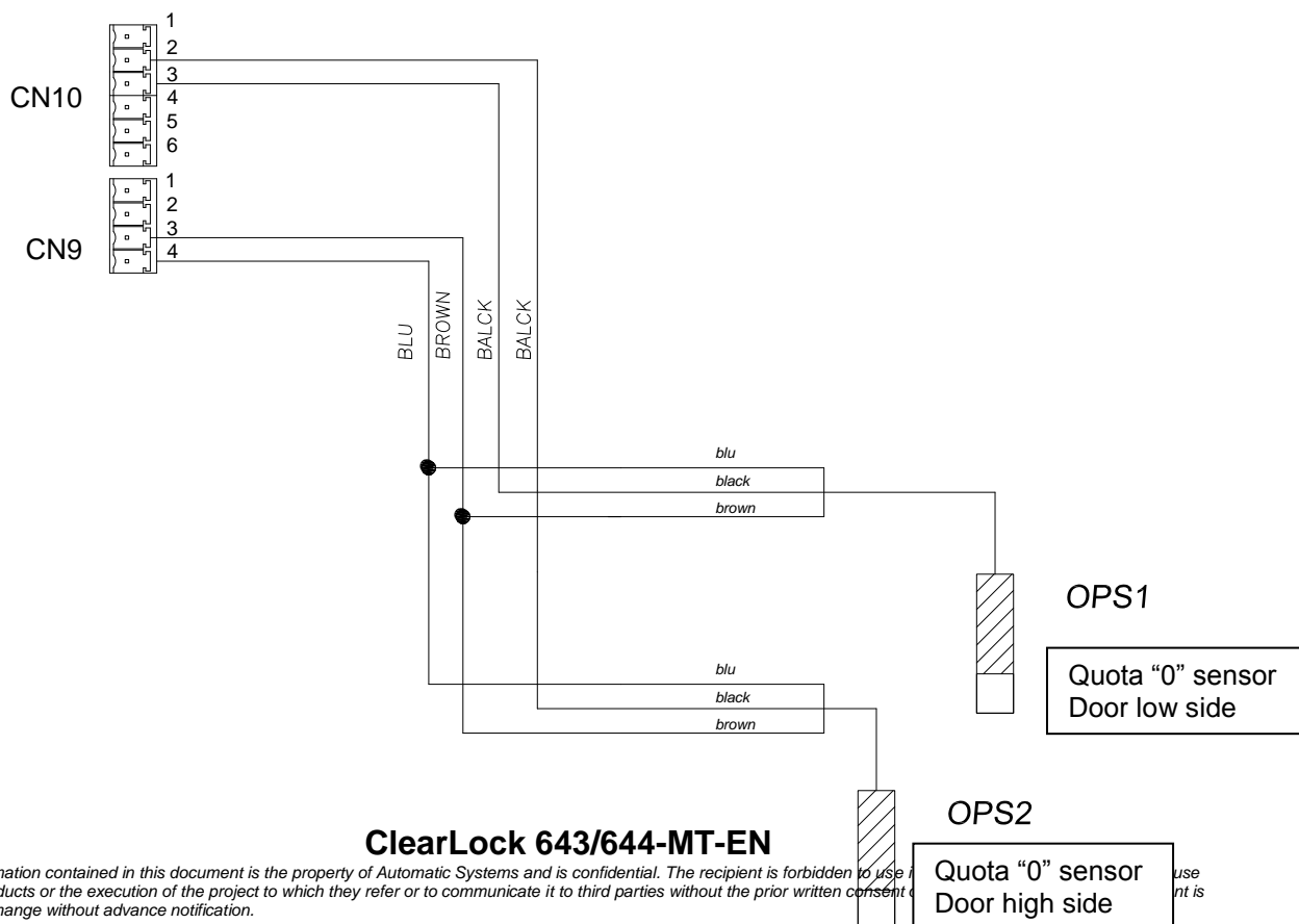
Figure 2-11 High and low side reset quota "0" sensor
