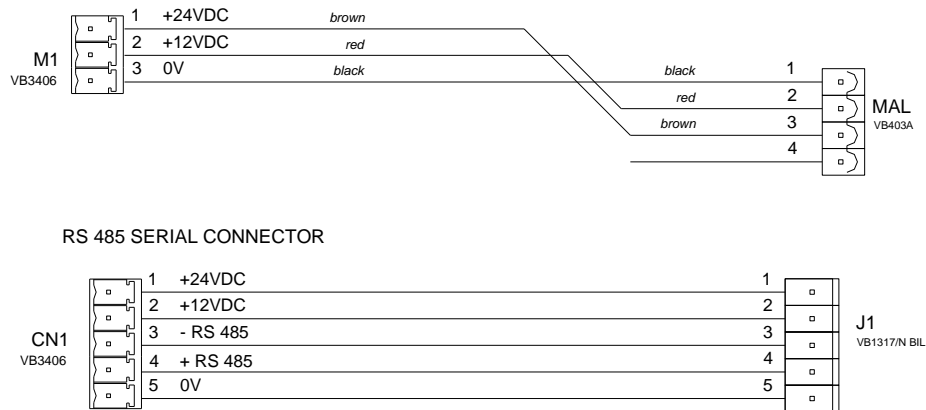
Figure 2-8 Metal detector wiring (if present)
