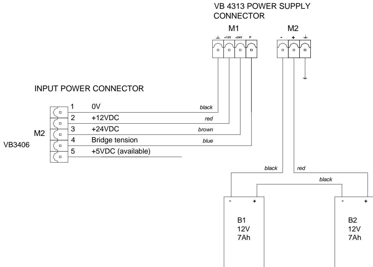
Figure 2-5 VB 4313SW Power supply wiring + Back-up batteries
