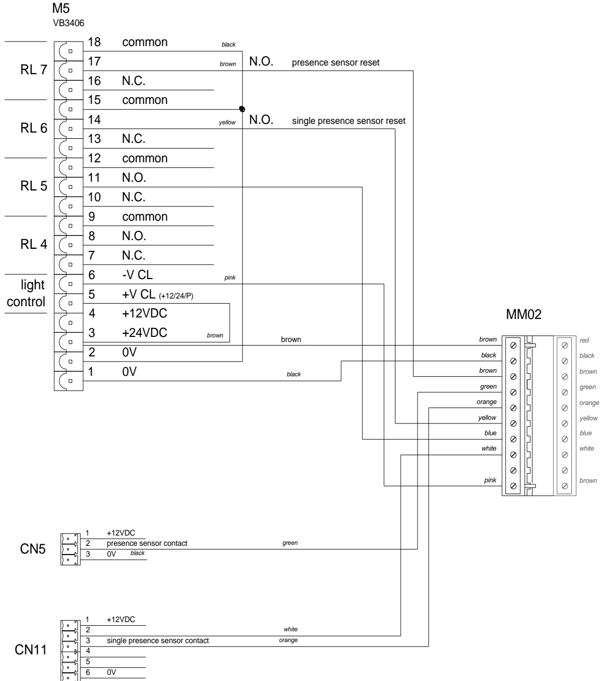
Figure 2-16 Connector MM02 wiring (part 1)
