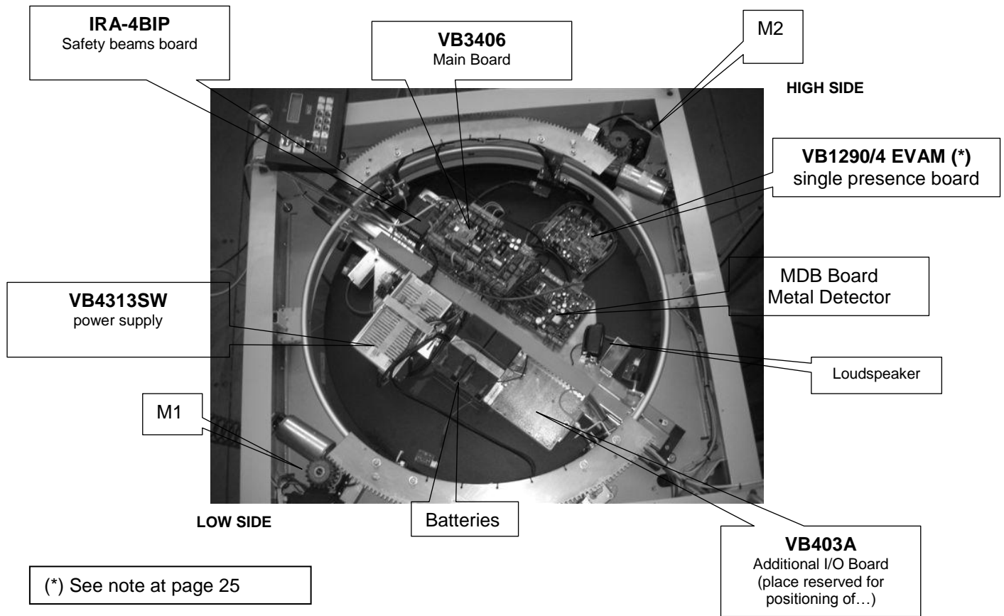
Figure 2-3 General components LAY OUT
