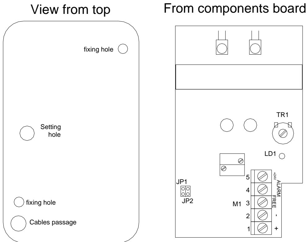
Figure 2-20 VB 2001 SD presence sensor
