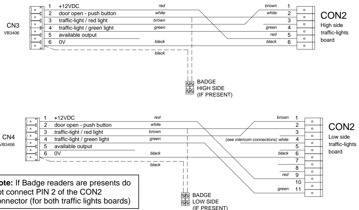
Figure 2-9 Traffic-light plate wiring
